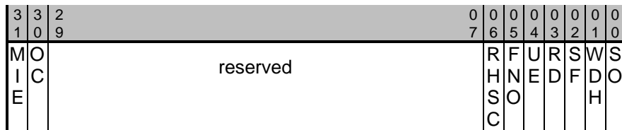
Figure 7-5: HcInterruptEnable Register
