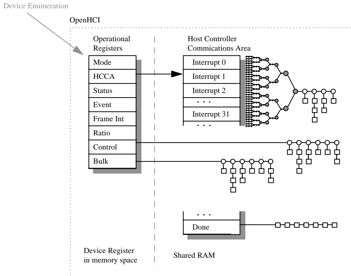
Figure 5-1: The OpenHCI Host Controller
