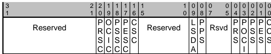
Figure 7-22: HcRhPortStatus Register
