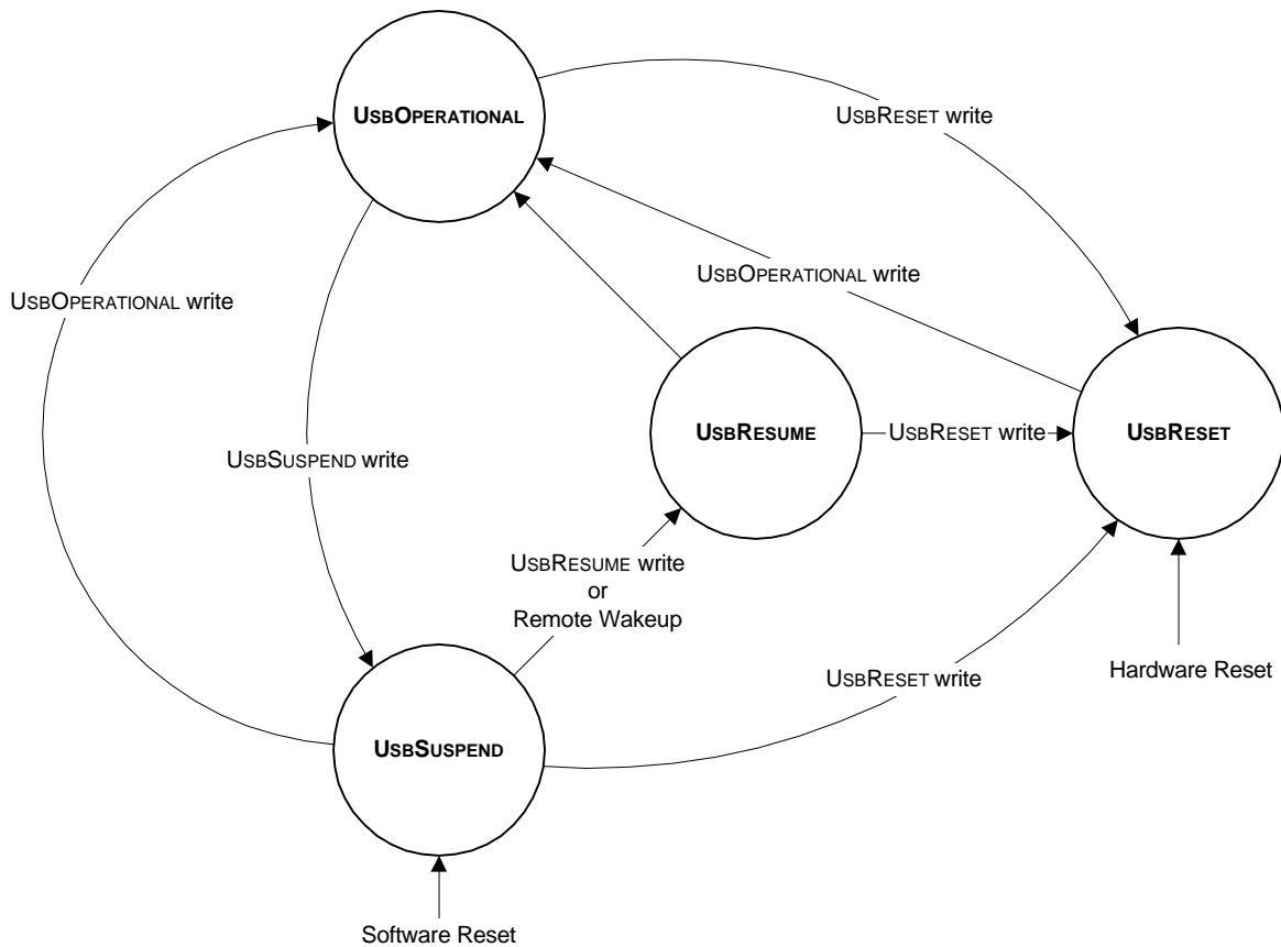
Figure 6-1: USB States
