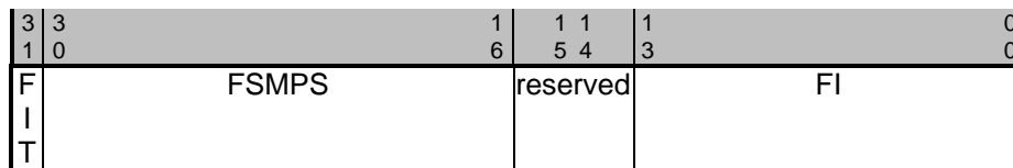
Figure 7-14: HcFmInterval Register
