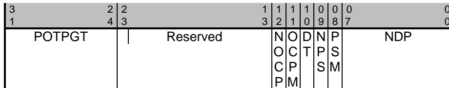
Figure 7-19: HcRhDescriptorA Register
