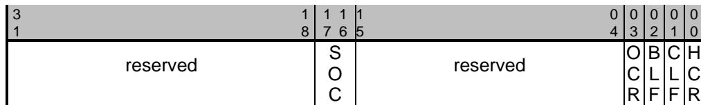
Figure 7-3: HcCommandStatus Register
